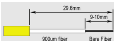
Note: The appropriate lengths of fiber and jacketing after cleaving. **Photo Not to Scale
