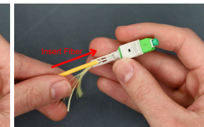
Step 11: Insert the fiber into the connector at a slight angle until the fibers meet.
